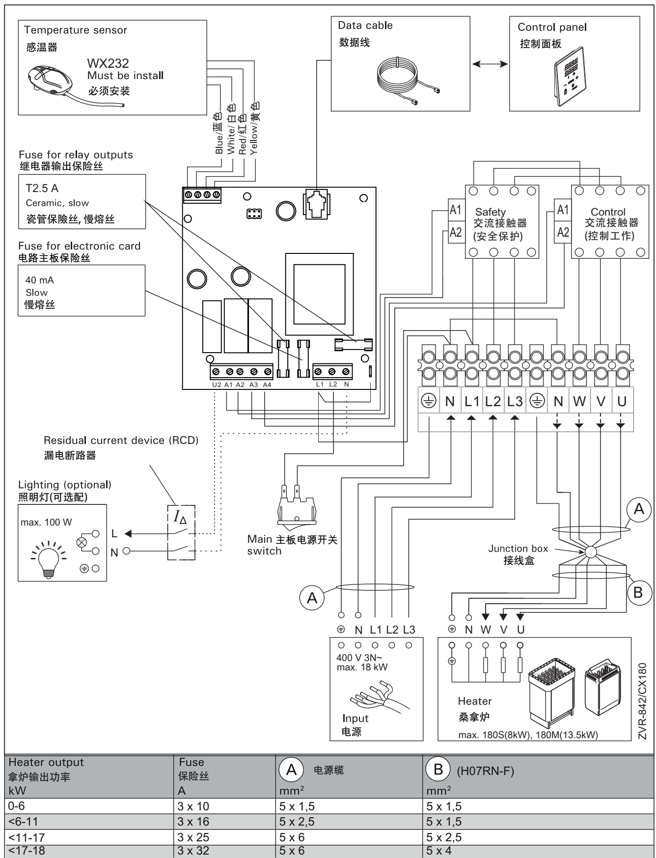
Figure 6a. CX180S, CX180M Electrical connections 图6a. CX180S, CX180M接线图
