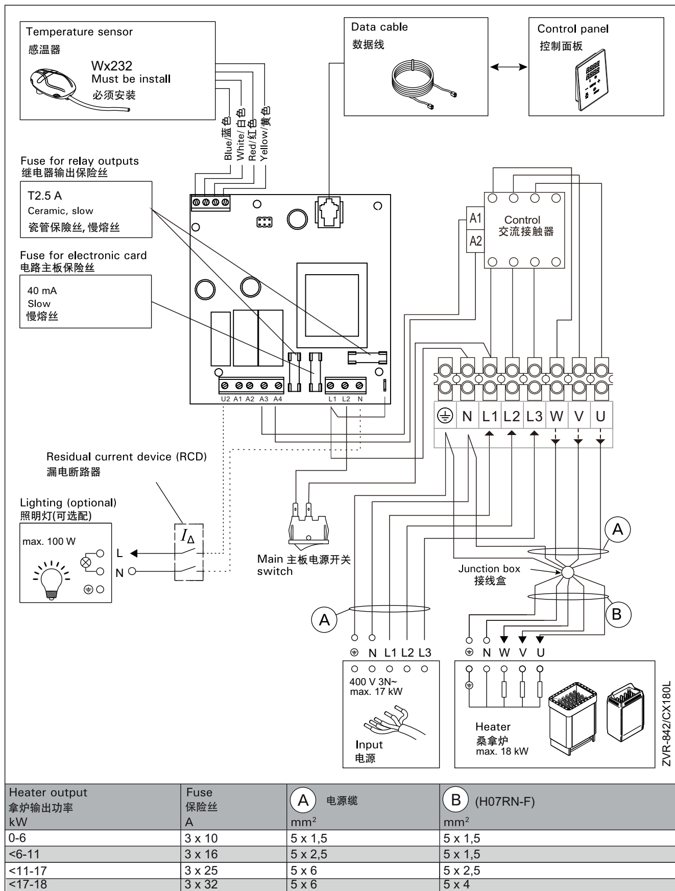
Figure 6b. CX180L Electrical connections 图6b. CX180L 接线图
